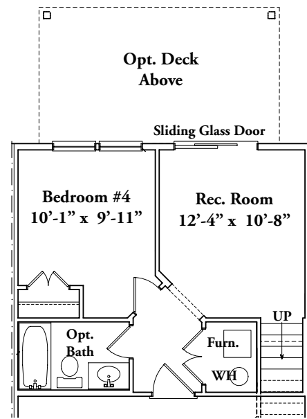
FIRST FLOOR PLAN W/ OPT. 4TH BEDROOM LAYOUT
