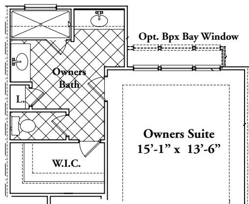
THIRD FLOOR PLAN MASTER BATH W/ SUNROOM BELOW
