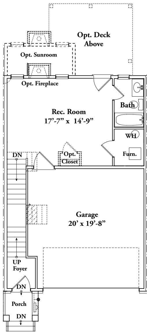
FIRST FLOOR PLAN SHOWN W/ OPT. SUNROOM
