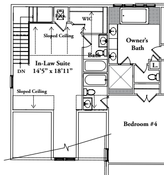
SECOND FLOOR W/ OPT. IN-LAW SUITE
