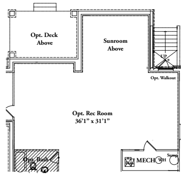
BASEMENT W/ OPT. SUNROOM AND DECK
