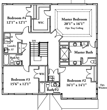
SECOND FLOOR W/ OPT. MASTER BATH LAYOUT
