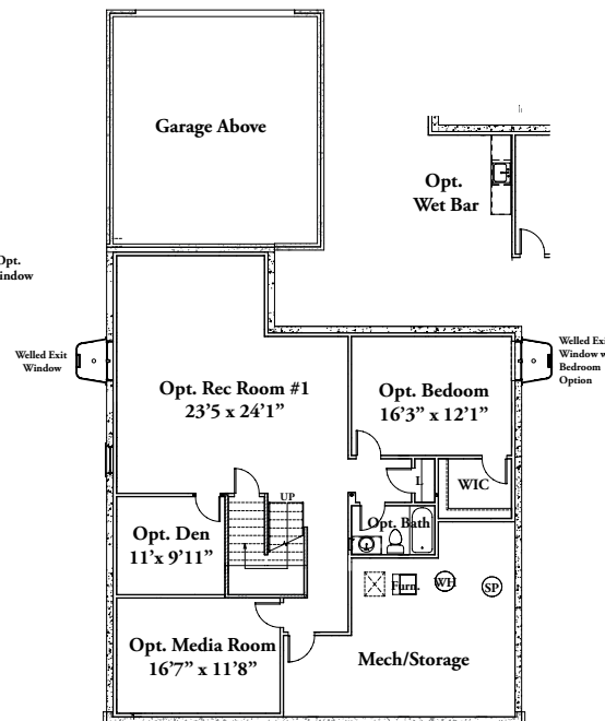
OPT. FINISHED BASEMENT
