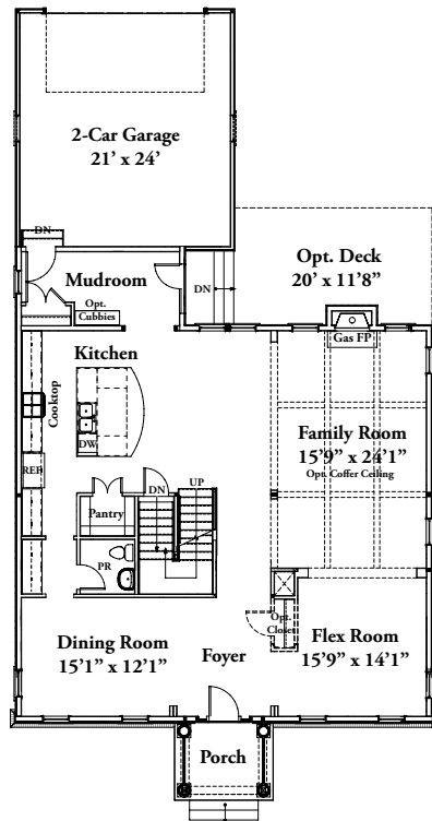
FIRST FLOOR - ELEV. 1
