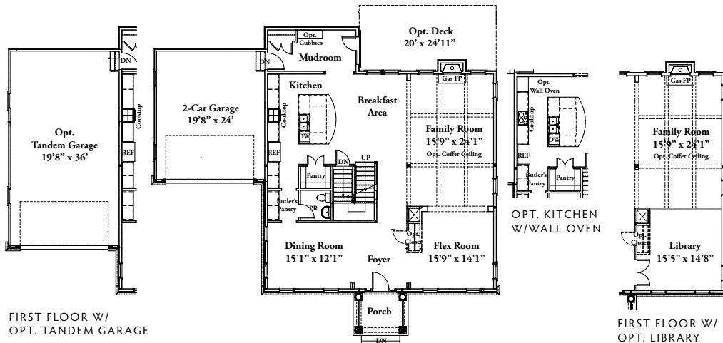
FIRST FLOOR - ELEV. 1
