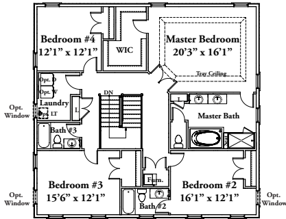
SECOND FLOOR - ELEV. 1 W/ STD. MASTER BATH LAYOUT
