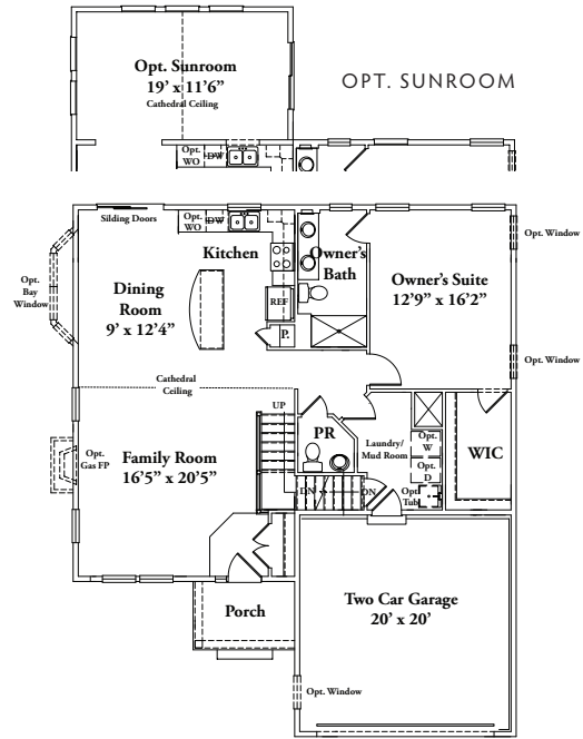
FIRST FLOOR - ELEV. 1 & 2
