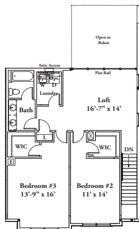
STD. SECOND FLOOR W/ OPT. LAUNDRY SHOWN AS RIGHT END UNIT
