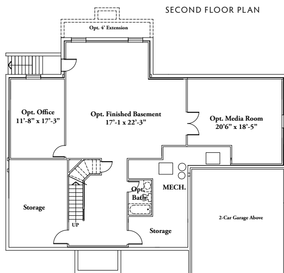
BASEMENT PLAN
