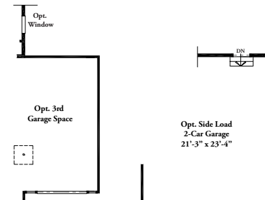
OPT. SIDE LOAD GARAGE
