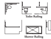
BATHROOM RAILING DETAIL
