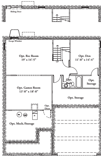
STANDARD BASEMENT PLAN
