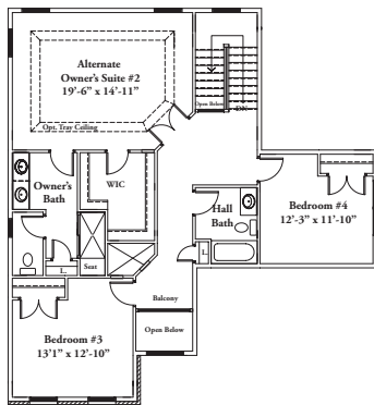
ALT. SECOND FLOOR W/ FOURTH BEDROOM
