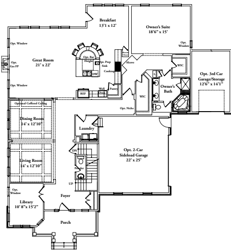
FIRST FLOOR - ELEV. 1 WITH OPT. 2-CAR SIDELOAD GARAGE AND OPT. 3RD CAR GARAGE
