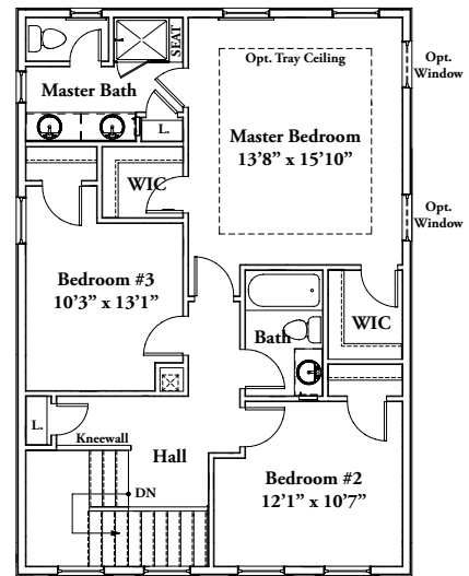
SECOND FLOOR - ELEV. 1
