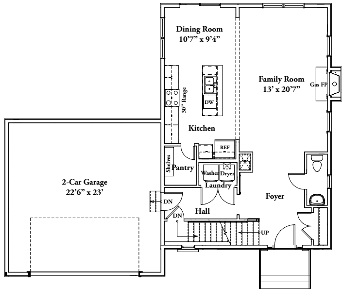
FIRST FLOOR - ELEV. 1
