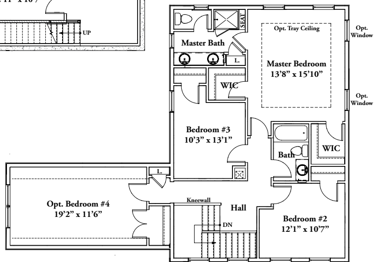
SECOND FLOOR SHOWN W/ OPT. BEDROOM #4
