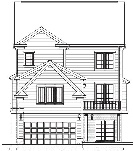
REAR ATTACHED GARAGE ELEVATION DETAIL
