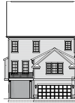
REAR ATTACHED GARAGE ELEVATION DETAIL
