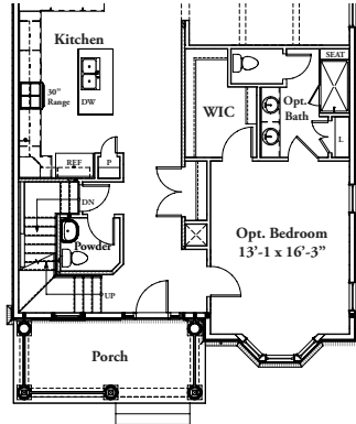
FIRST FLOOR - ELEV. 1 W/ OPT. BEDROOM
