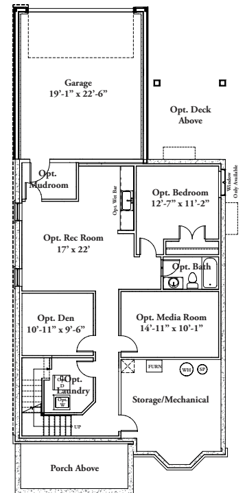
OPT. FINISHED BASEMENT PLAN W/ ATTACHED BASEMENT GARAGE (SITE SPECIFIC)
