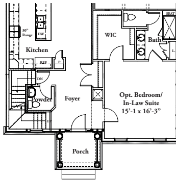
FIRST FLOOR - ELEV. 1 W/ OPT. BEDROOM/IN-LAW SUITE
