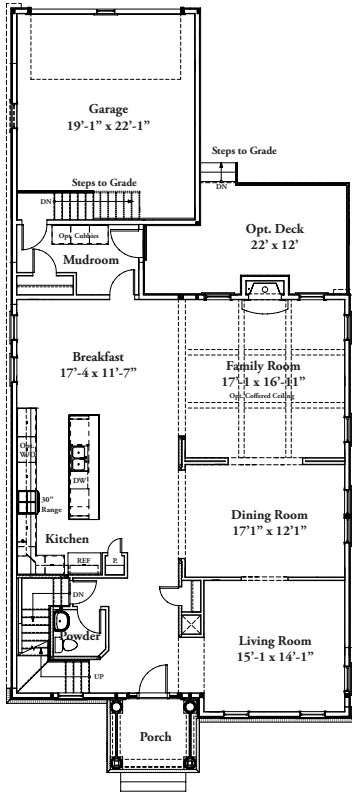
FIRST FLOOR - ELEV. 1 W/ ATTACHED GARAGE
