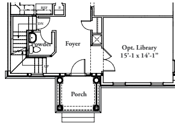
FIRST FLOOR - ELEV. 1 W/ OPT. LIBRARY
