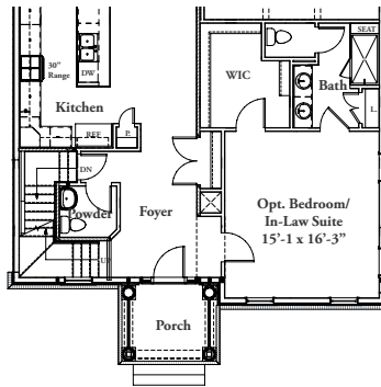
FIRST FLOOR - ELEV. 1 W/ OPT. BEDROOM/IN-LAW SUITE
