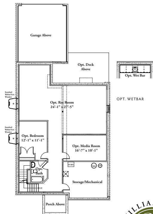
OPT. FINISHED BASEMENT PLAN
