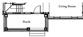
FIRST FLOOR - ELEV. 3
