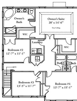
OPTIONAL SECOND FLOOR W/ 3 BATHROOMS
