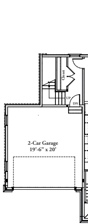
FIRST FLOOR W/ 2-CAR FRONT LOAD GARAGE W/ STAIRS TO OPT. BONUS ROOM
