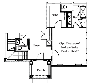
FIRST FLOOR - ELEV. 1 W/ OPT. BEDROOM/IN-LAW SUITE
