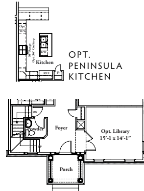
FIRST FLOOR - ELEV. 1 W/ OPT. LIBRARY
