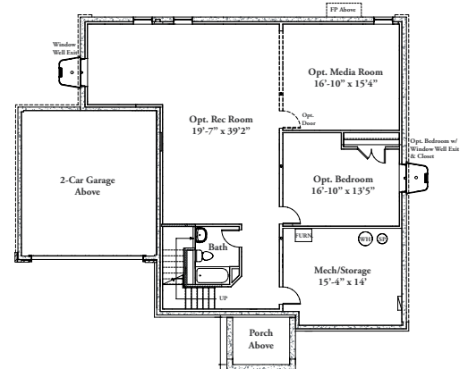
OPT. FINISHED BASEMENT PLAN
