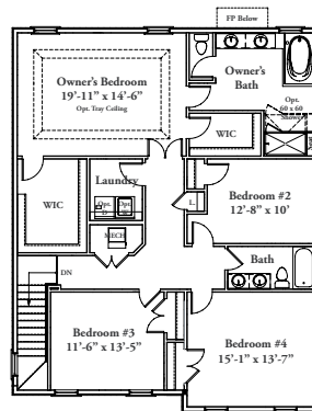
STANDARD SECOND FLOOR
