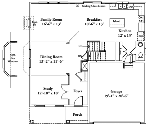
FIRST FLOOR - ELEV. 1
