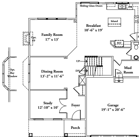
FIRST FLOOR W/ OPTIONAL 6' REAR EXT.
