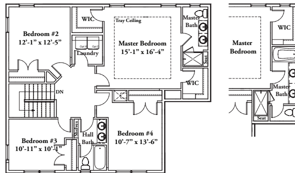
SECOND FLOOR - ELEV. 1&2
