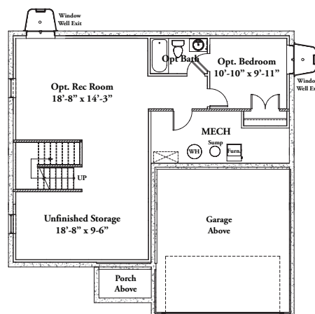
BASEMENT - ELEV. 1&2
