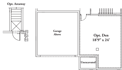
OPT. DEN W/ EXTENSION
