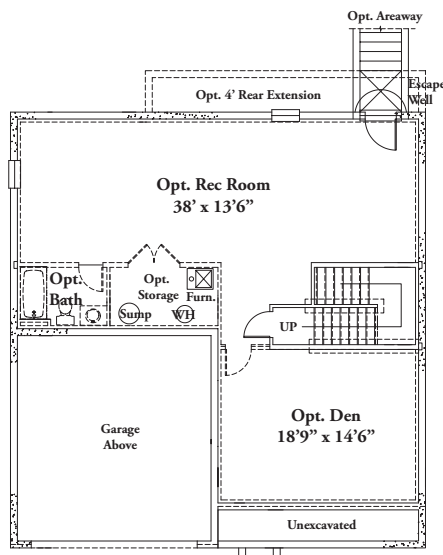
BASEMENT - ELEV. 1 & 2
