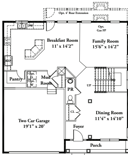
FIRST FLOOR - ELEV. 1 & 2
