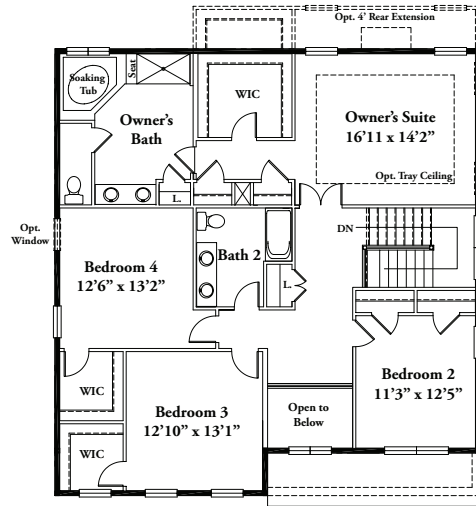
SECOND FLOOR - ELEV. 1 & 2
