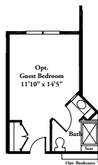
FIRST FLOOR PLAN W/ OPT. GUEST BEDROOM & FULL BATH (IN LIEU OF LIBRARY)
