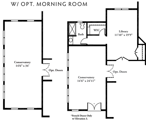
FIRST FLOOR PLAN W/ OPT. 2- STORY CONSERVATORY
