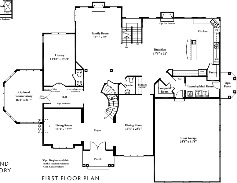
FIRST FLOOR PLAN W/ OPT. CONSERVATORY
