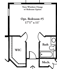
SECOND FLOOR PLAN W/ OPT. BEDROOM #5 ABOVE FAMILY ROOM
