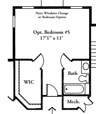
SECOND FLOOR PLAN W/ OPT. BEDROOM #5 ABOVE FAMILY ROOM
