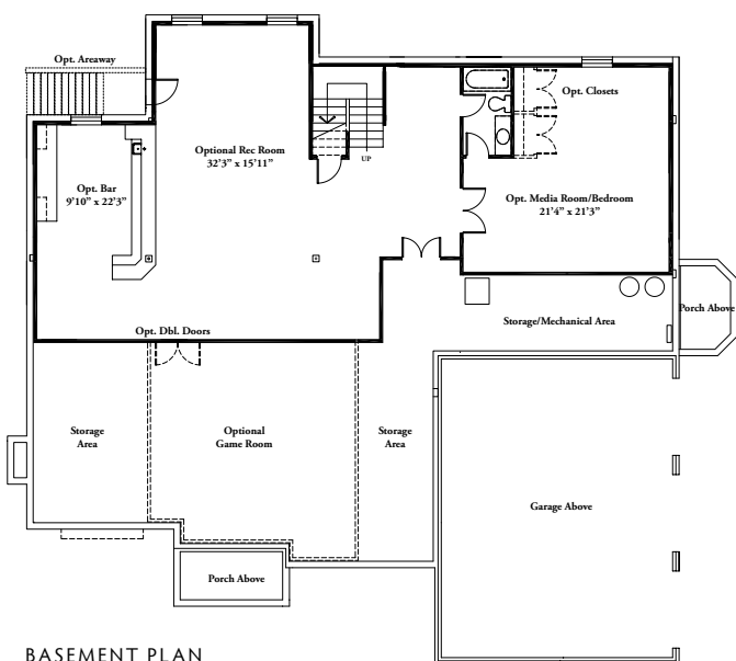
BASEMENT PLAN
