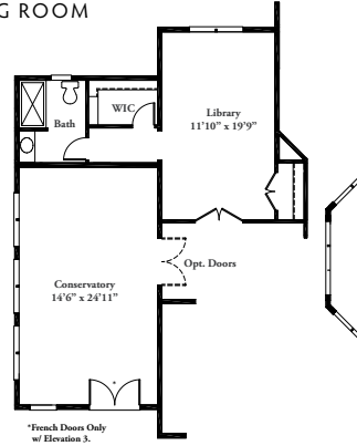
FIRST FLOOR PLAN W/ OPT. FULL BATH, LIBRARY AND OPT. 2-STORY CONSERVATORY
