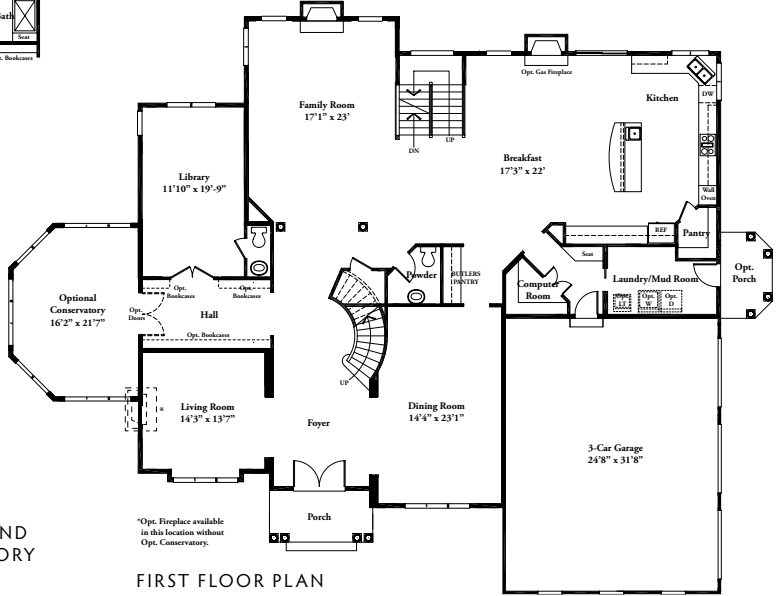
FIRST FLOOR PLAN W/ OPT. CONSERVATORY
