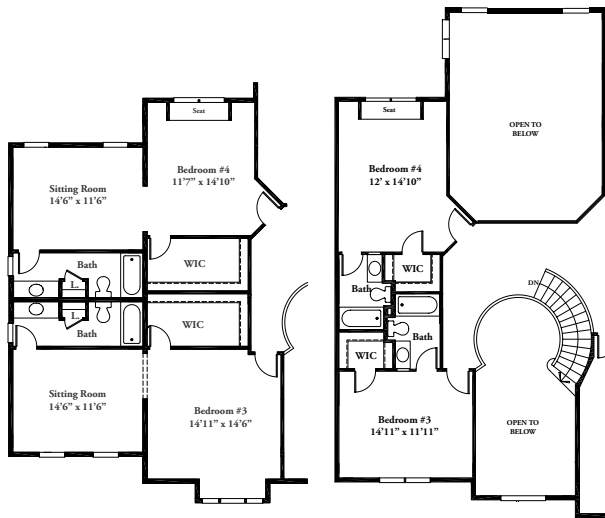
SECOND FLOOR PLAN W/ 2-STORY CONSERVATORY
